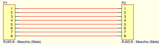
CBL057A000 - RJ45-8/RJ45-8 one to one cable - L=30 cm
