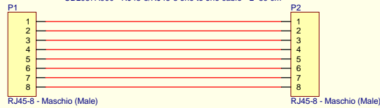
CBL057A300 - RJ45-8/RJ45-8 one to one cable - L= 2 mt
