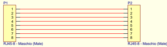
CBL057A500 - RJ45-8/RJ45-8 one to one cable - L= 6 mt
